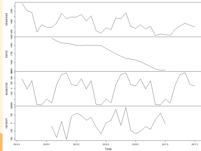
Decomposition of additive time series
